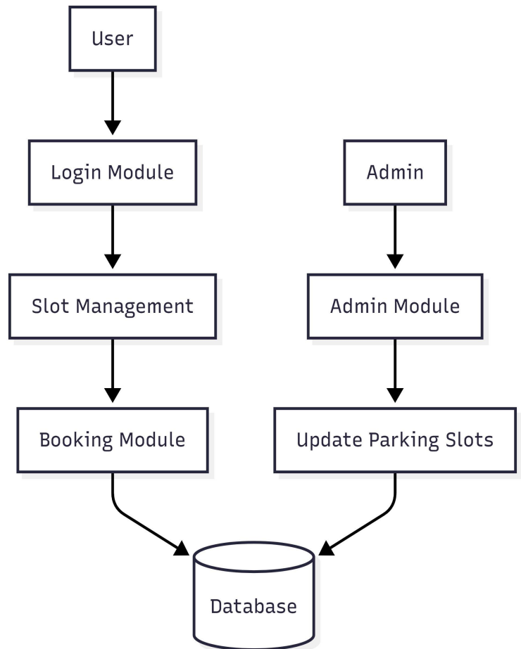
Fig. 3. Data Flow Diagram – Level 1
