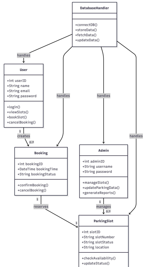
Fig. 5. UML Class Diagram
