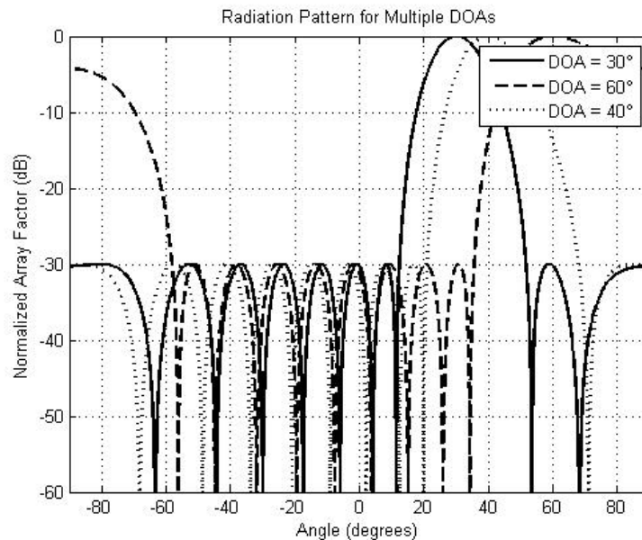
Figure 2: Radiation Pattern For DOA= 30^\circ , 60^\circ , 40^\circ
