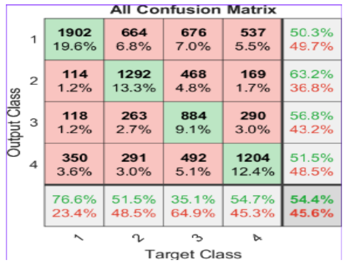
Fig 9: Confusion matrix of model trained by features extracted from edge detection model
