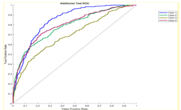
Fig 11: ROC curve of model trained by features extracted from edge detection method
